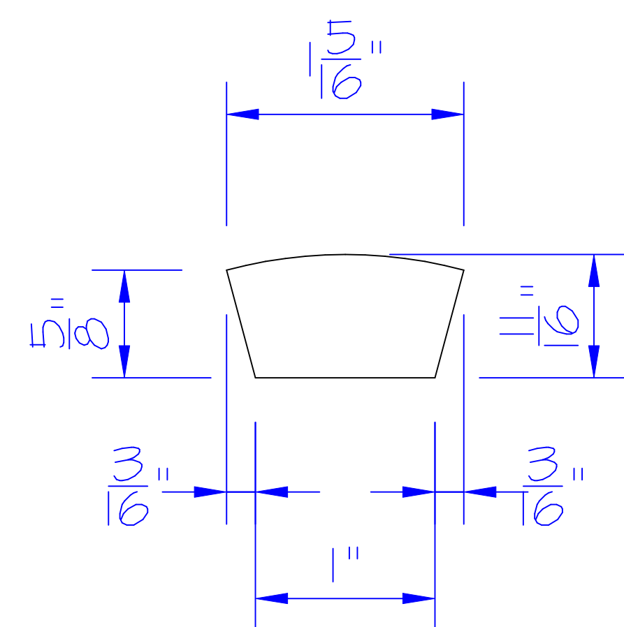
END VIEW
