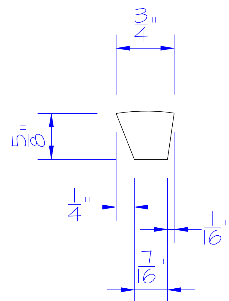
END VIEW
