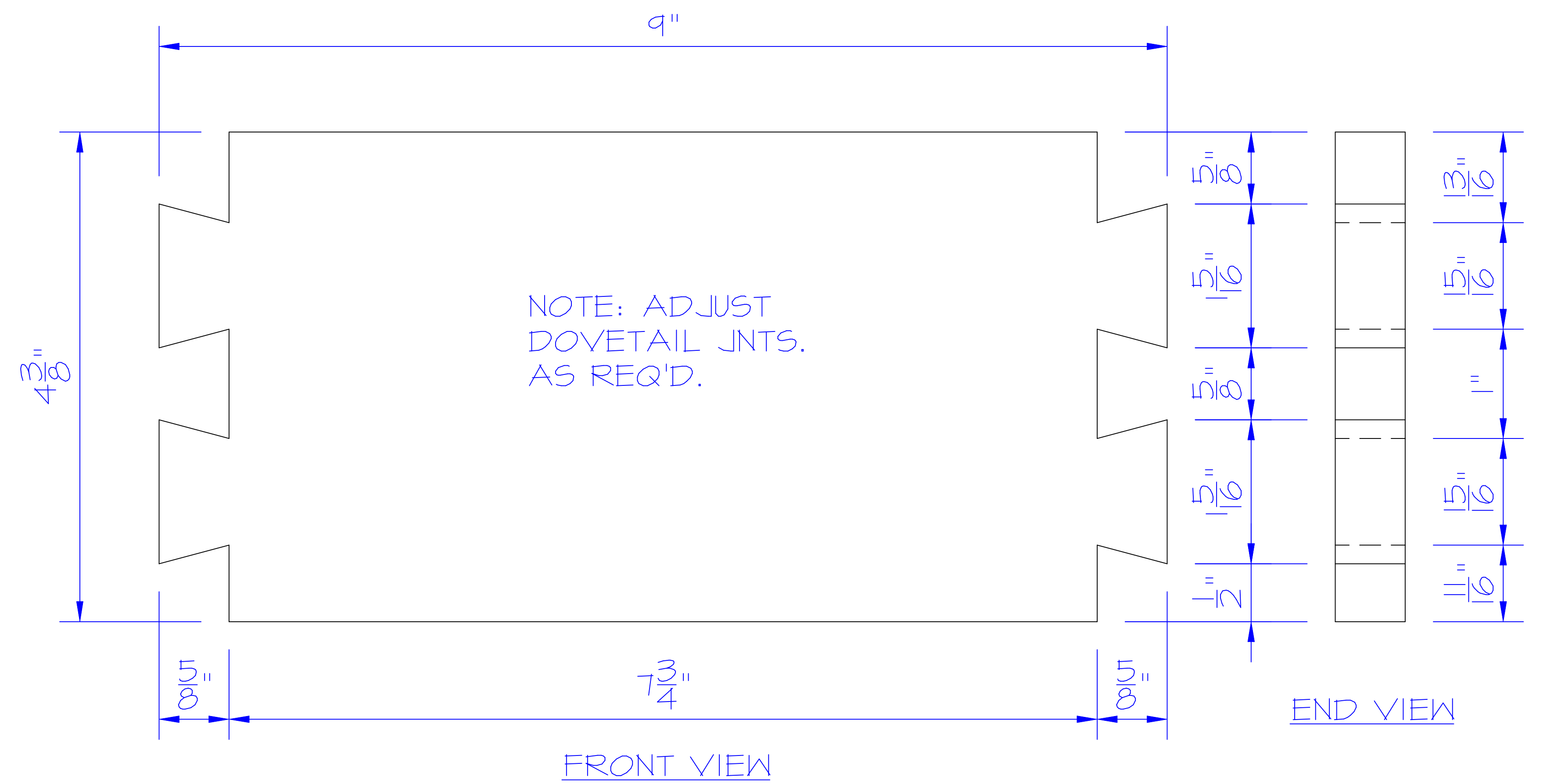
FRONT & BACK BOARD 2 NEEDED
