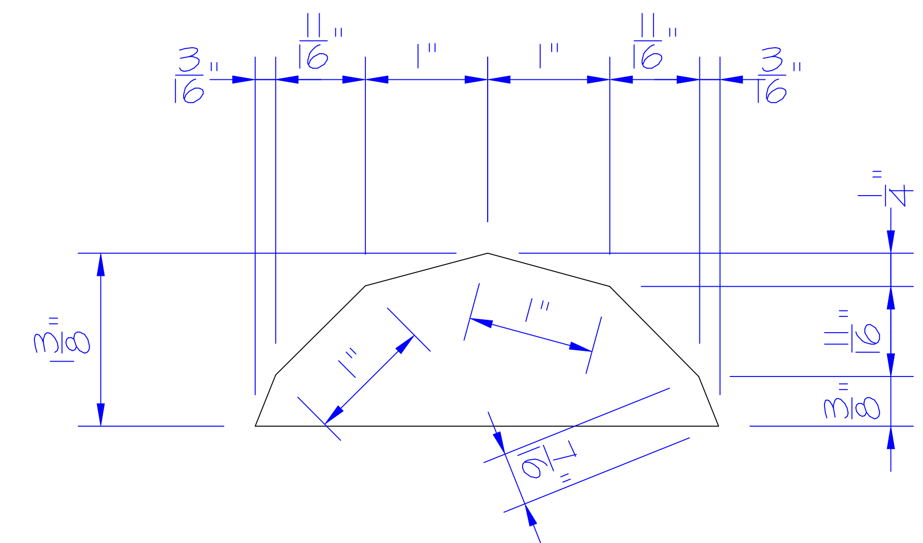
LID SIDE BOARD 2 NEEDED
