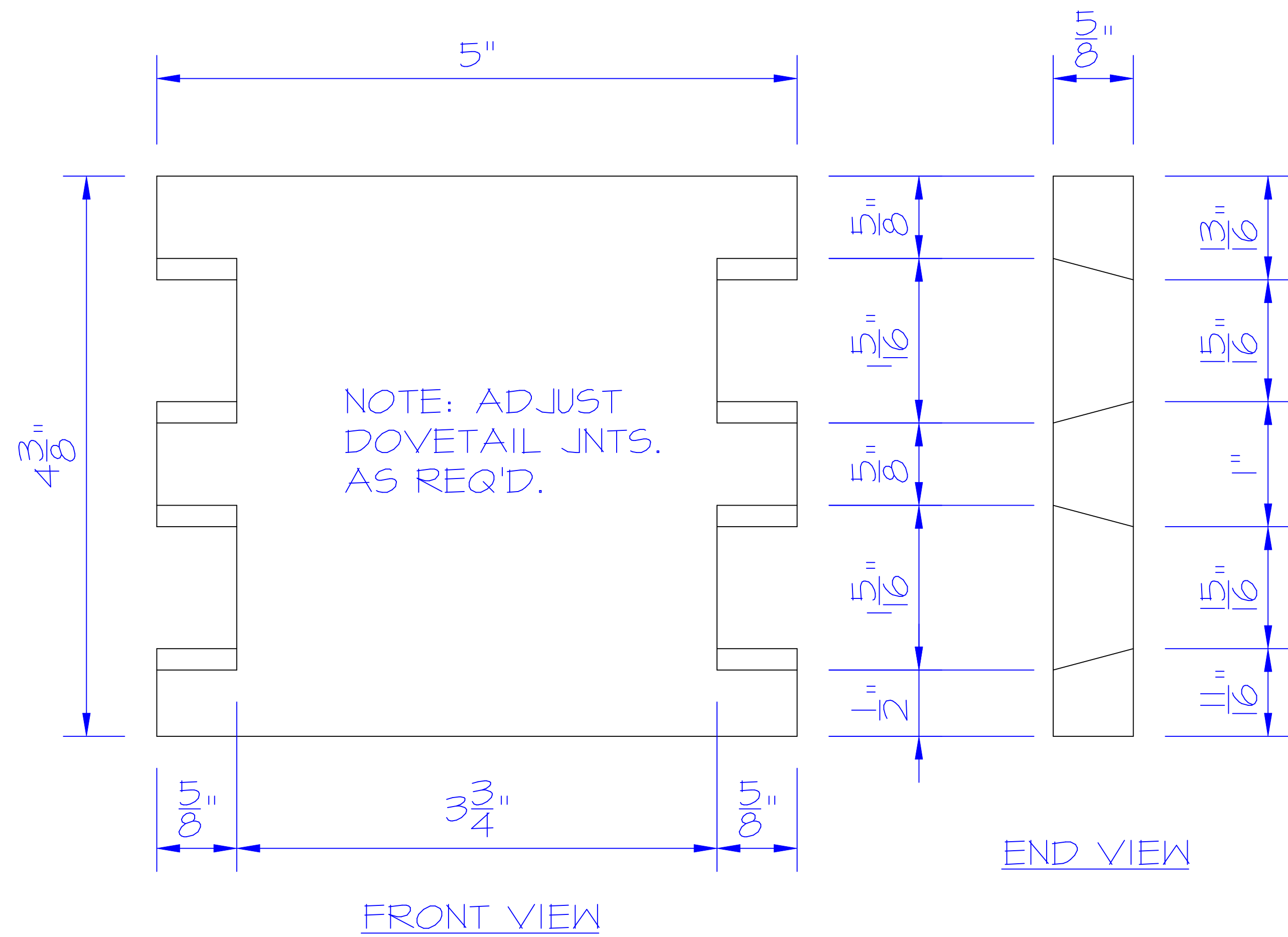
SIDE BOARD 2 NEEDED
