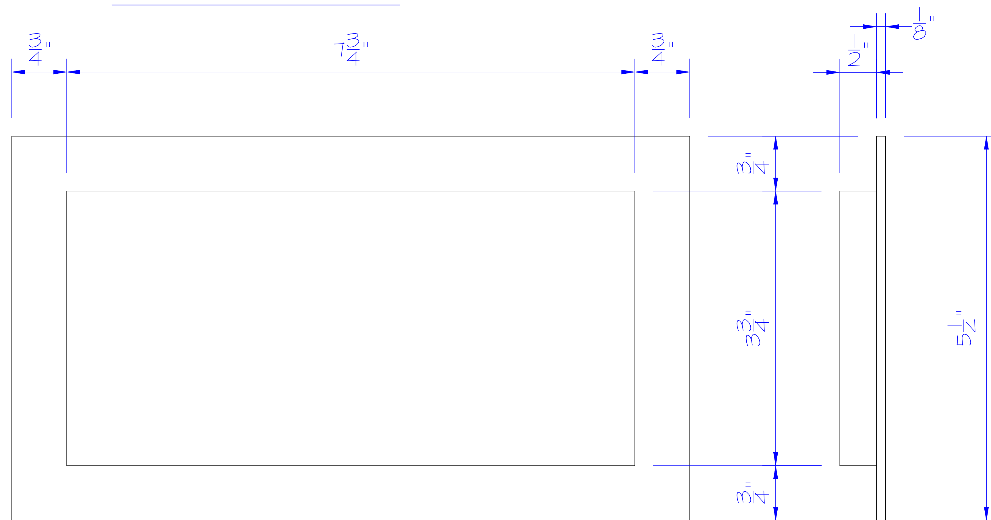
SIDE BOARD 2 NEEDED
